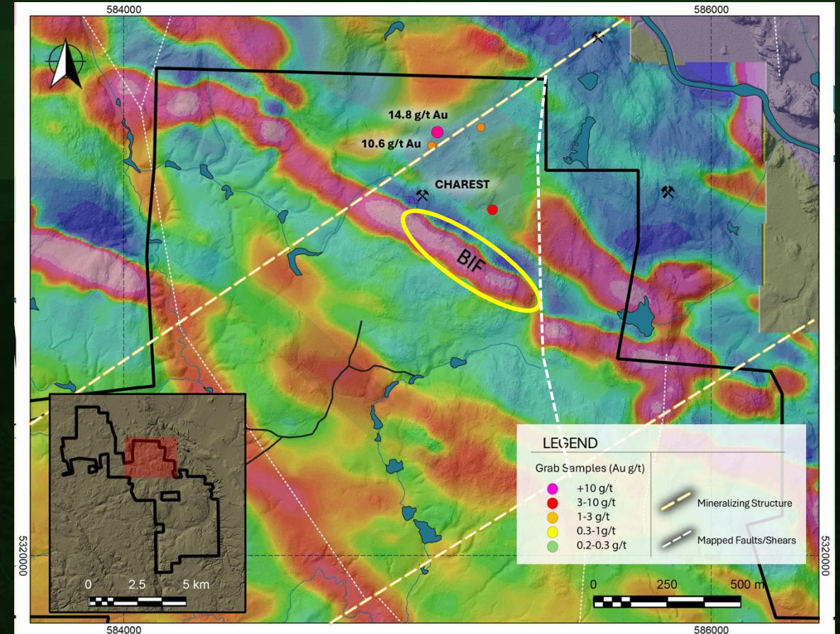
2026 Expert - CVG-TMI (Calculated Vertical Gradient of Total Magnetic Intensity)
